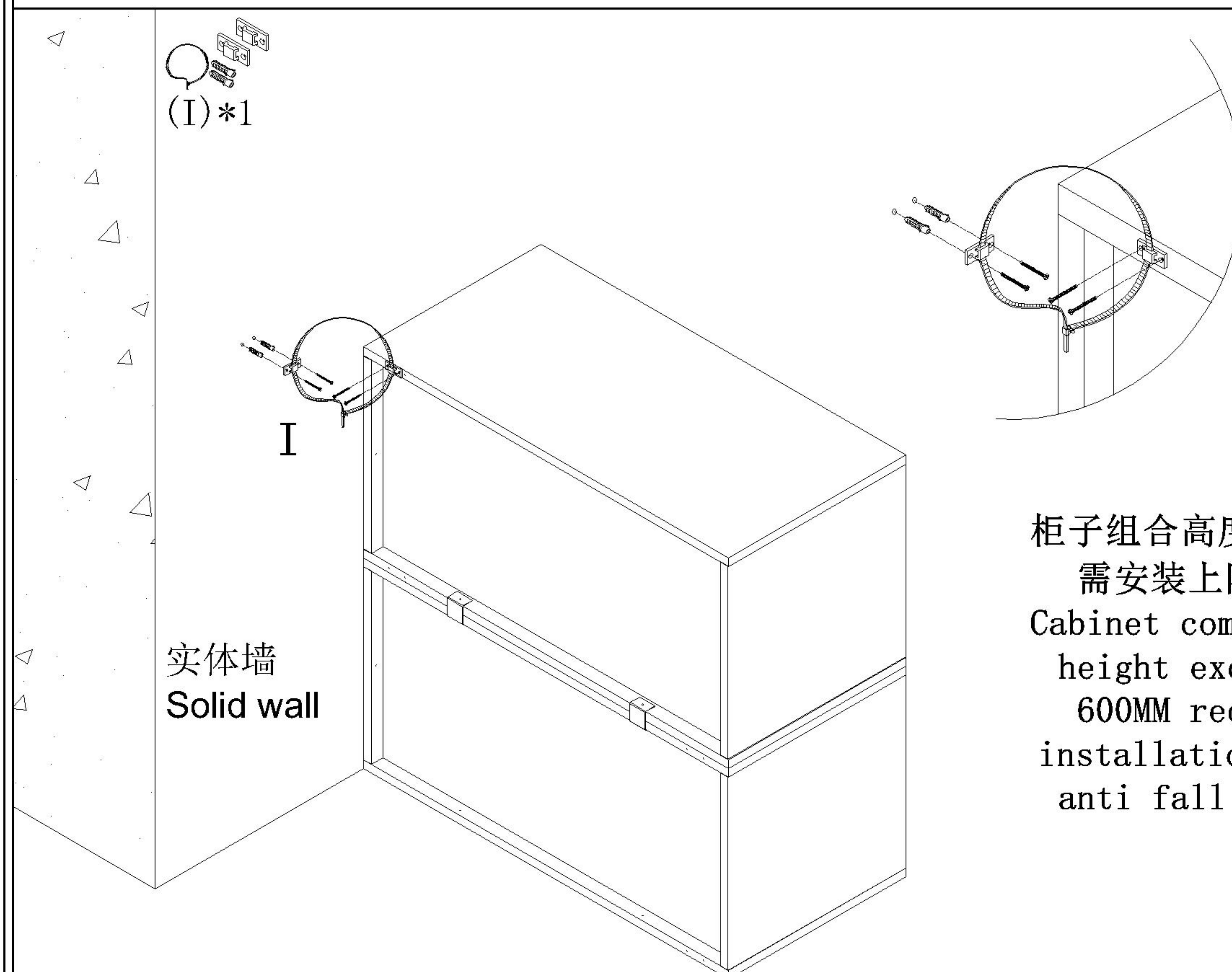
上下组合安装方式 Upper and lower combination installation method
