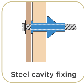
Self-drill fixing
