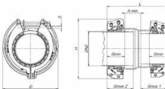
1 bolt pr. side DN40-DN200
