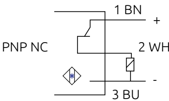
wiring diagram
