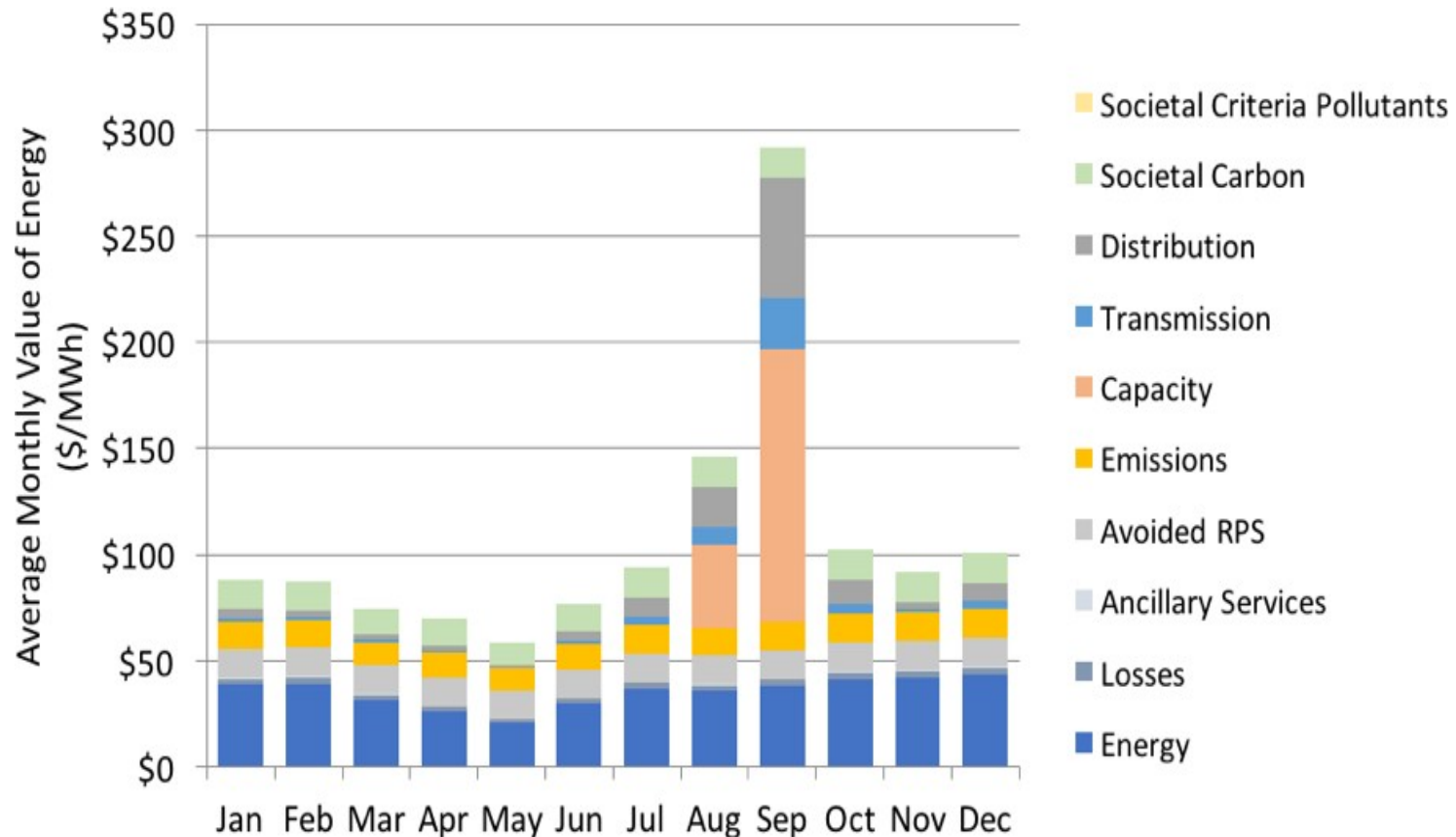
East Bay region, Climate Zone (CZ) 3A, Western Alameda County
