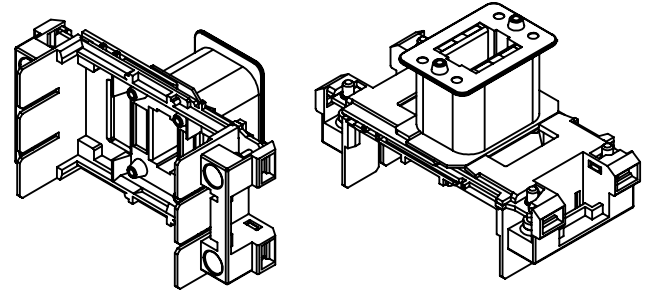
ISO VIEW
