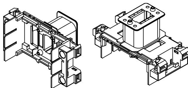
ISO VIEW
