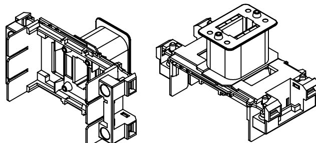
ISO VIEW
