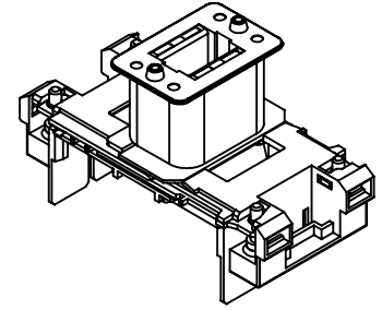
ISO VIEW
