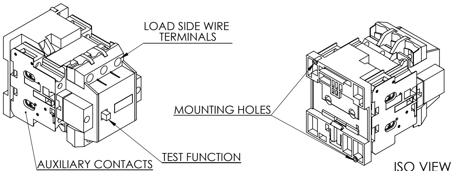
ISO VIEW
