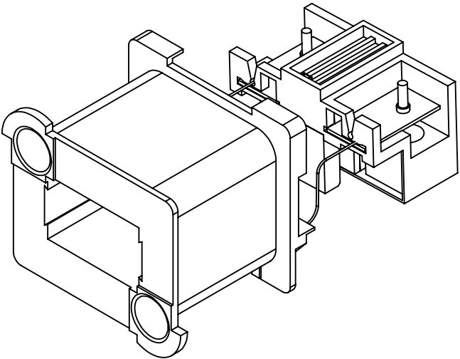
ISO VIEW
