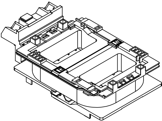
ISO VIEW
