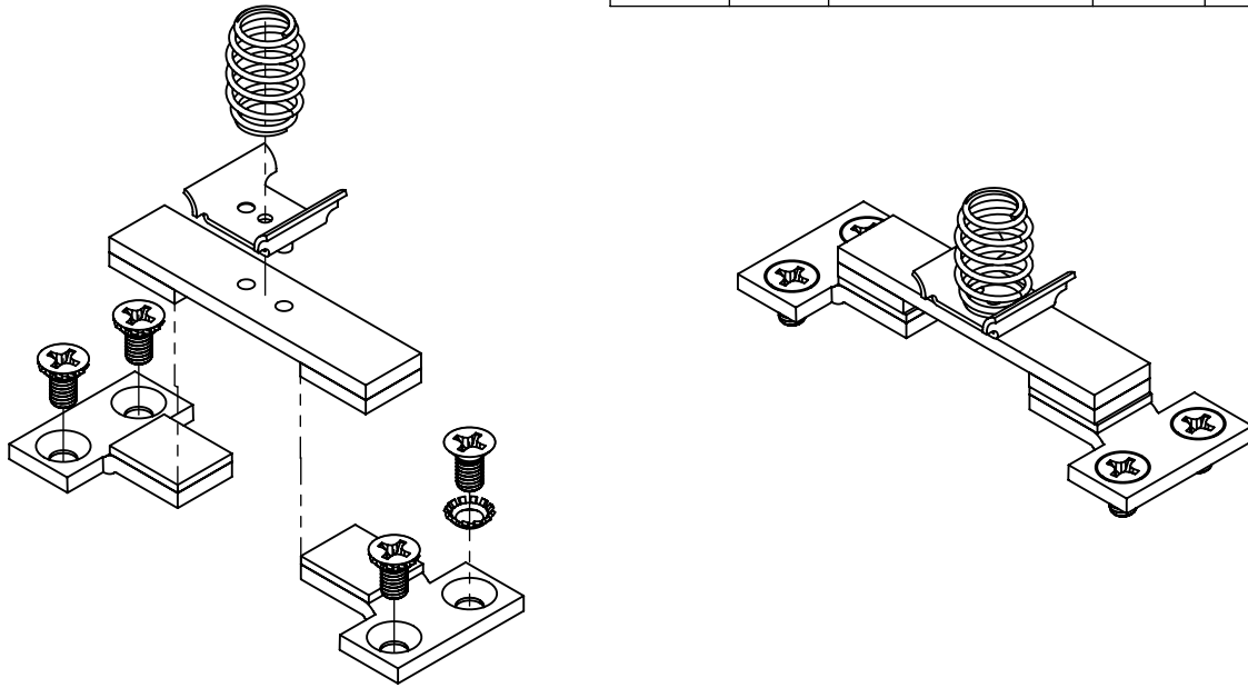
EXPLODED VIEW
