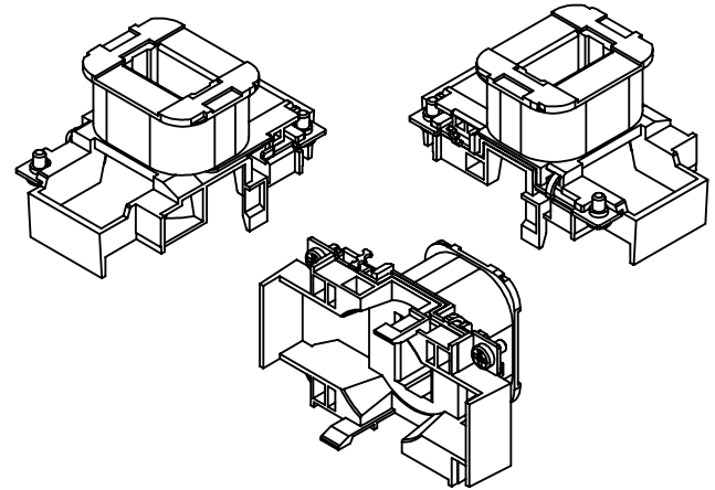
ISO VIEW
