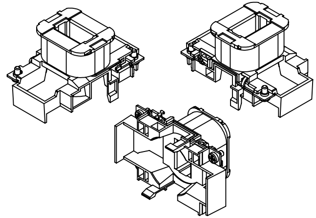
ISO VIEW
