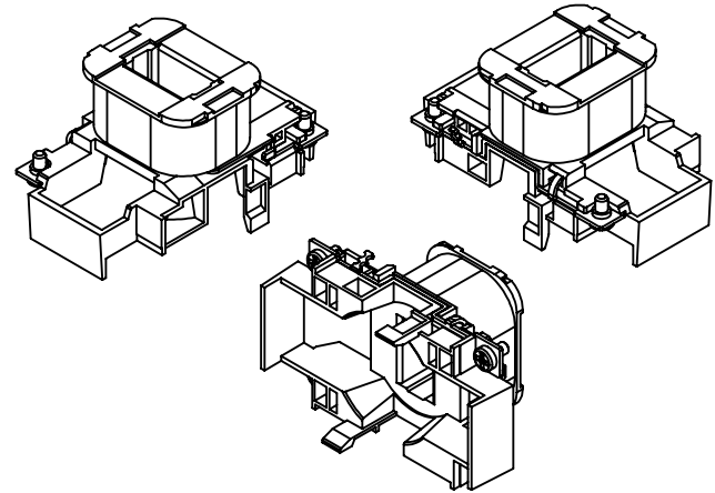
ISO VIEW
