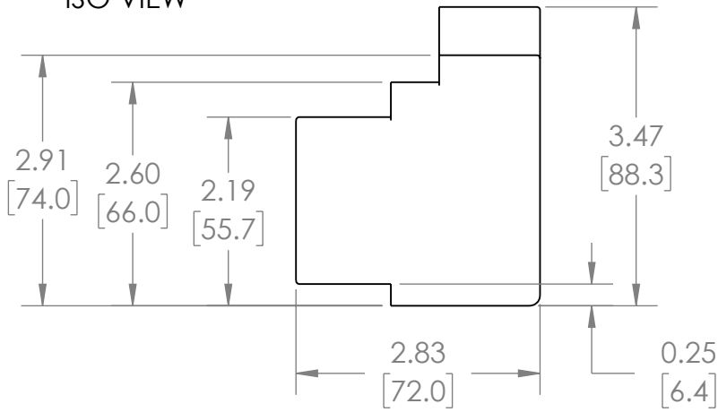
ISO VIEW
