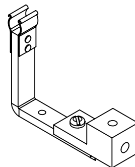
ISO VIEW
