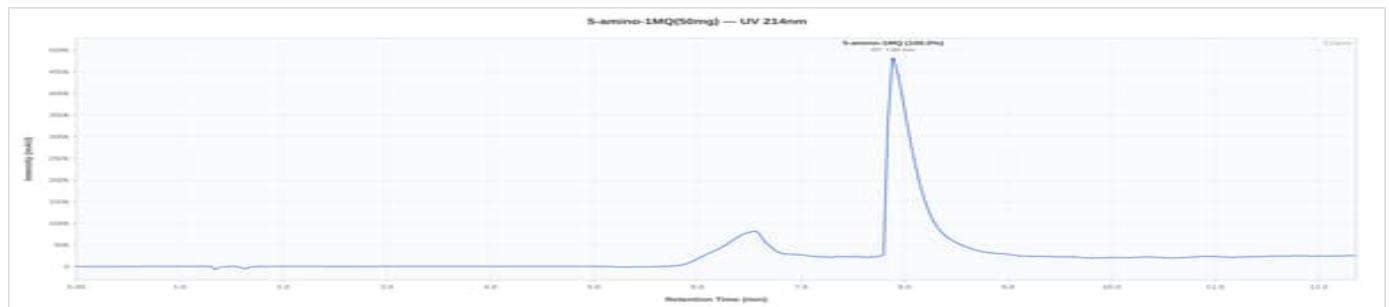
5-Amino-1q 50mg - 5AMQ904PTR: UV Chromatogram
