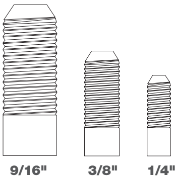
RIGHT-HAND THREADS
