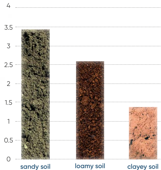
Corrosion rate improvement with Magnelis ® versus post-galvanised steel
