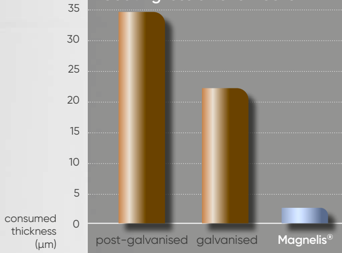
Coating loss after 6 weeks
