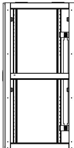
Side View without Side Panels
