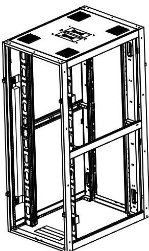
Isometric View without doors, side panels
