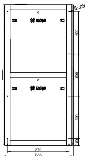
Side View with Side Panels
