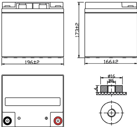
Unit:(mm) Terminal type:(T1)
