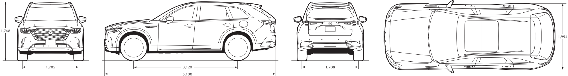
DIMENSIONS (mm)
