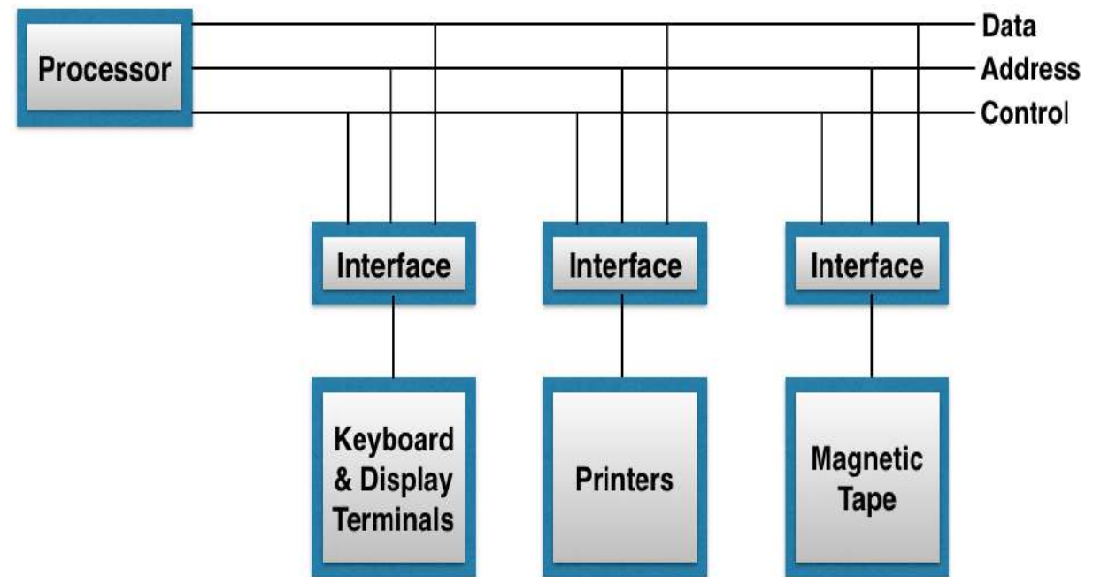
Connection of I/O Bus to I/O Device
