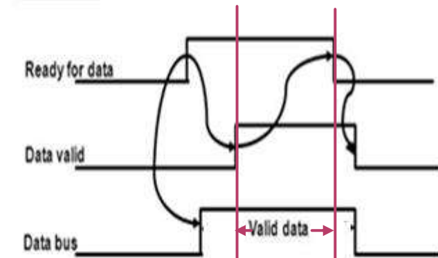
Timing Diagram
