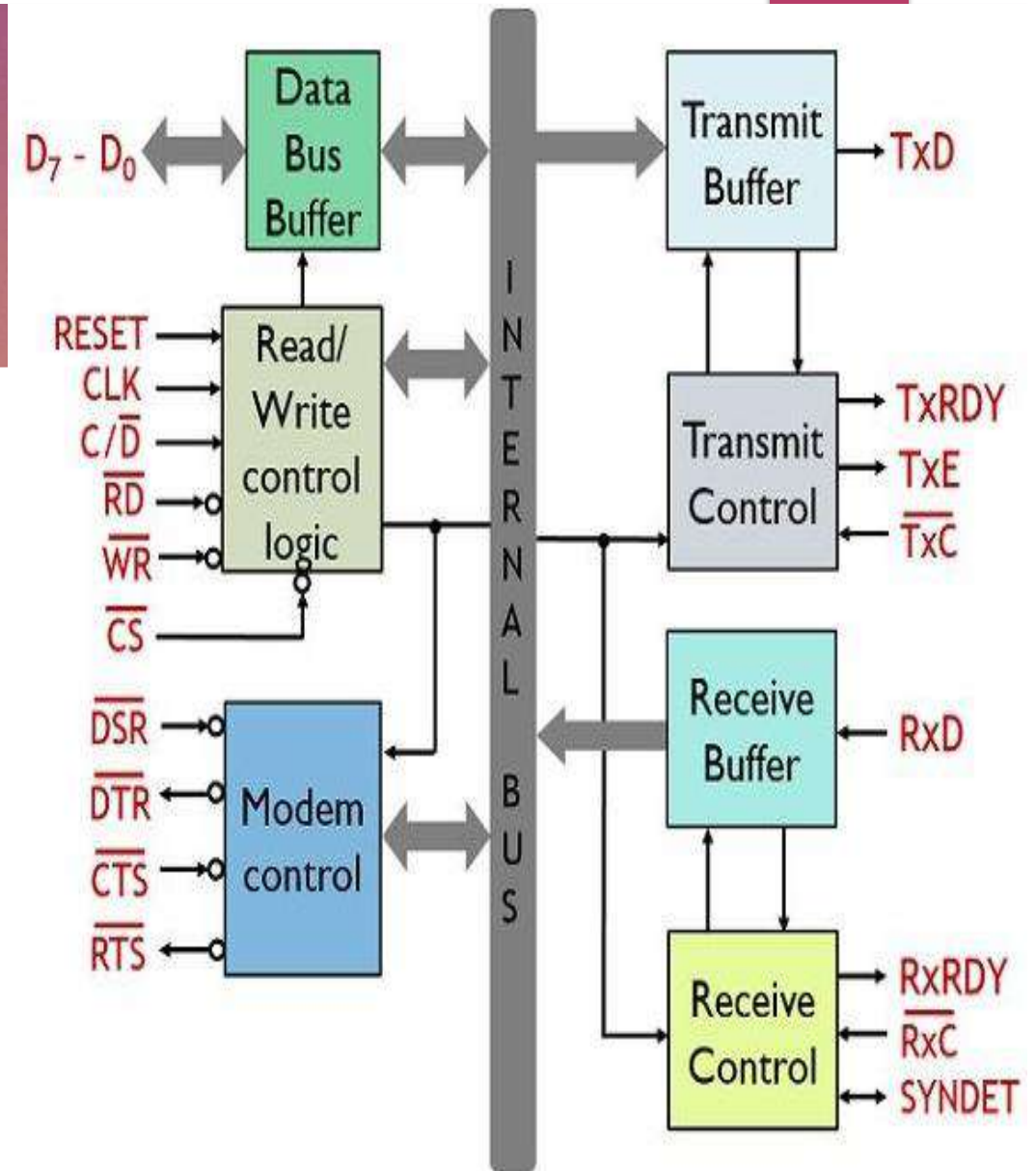
Architecture of 8251 USART
