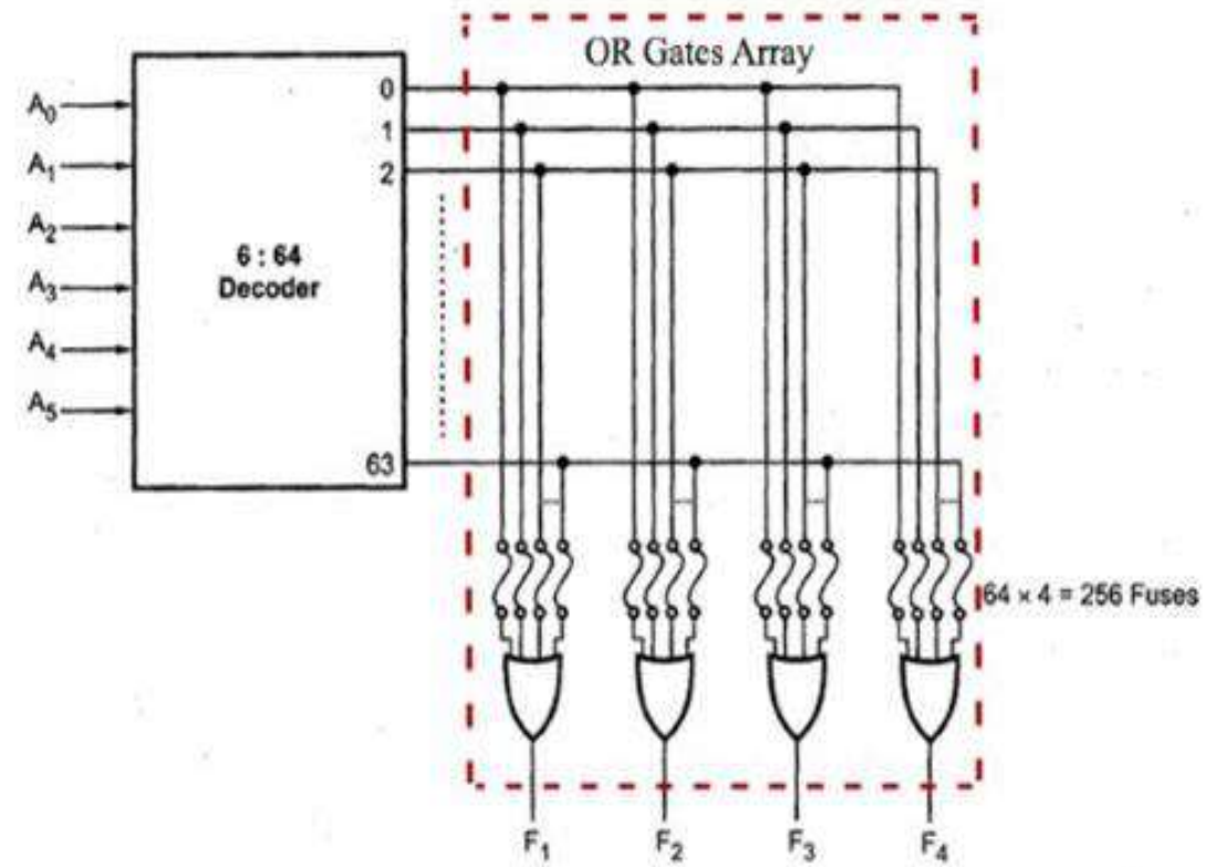
Internal construction of 64x4 ROM
