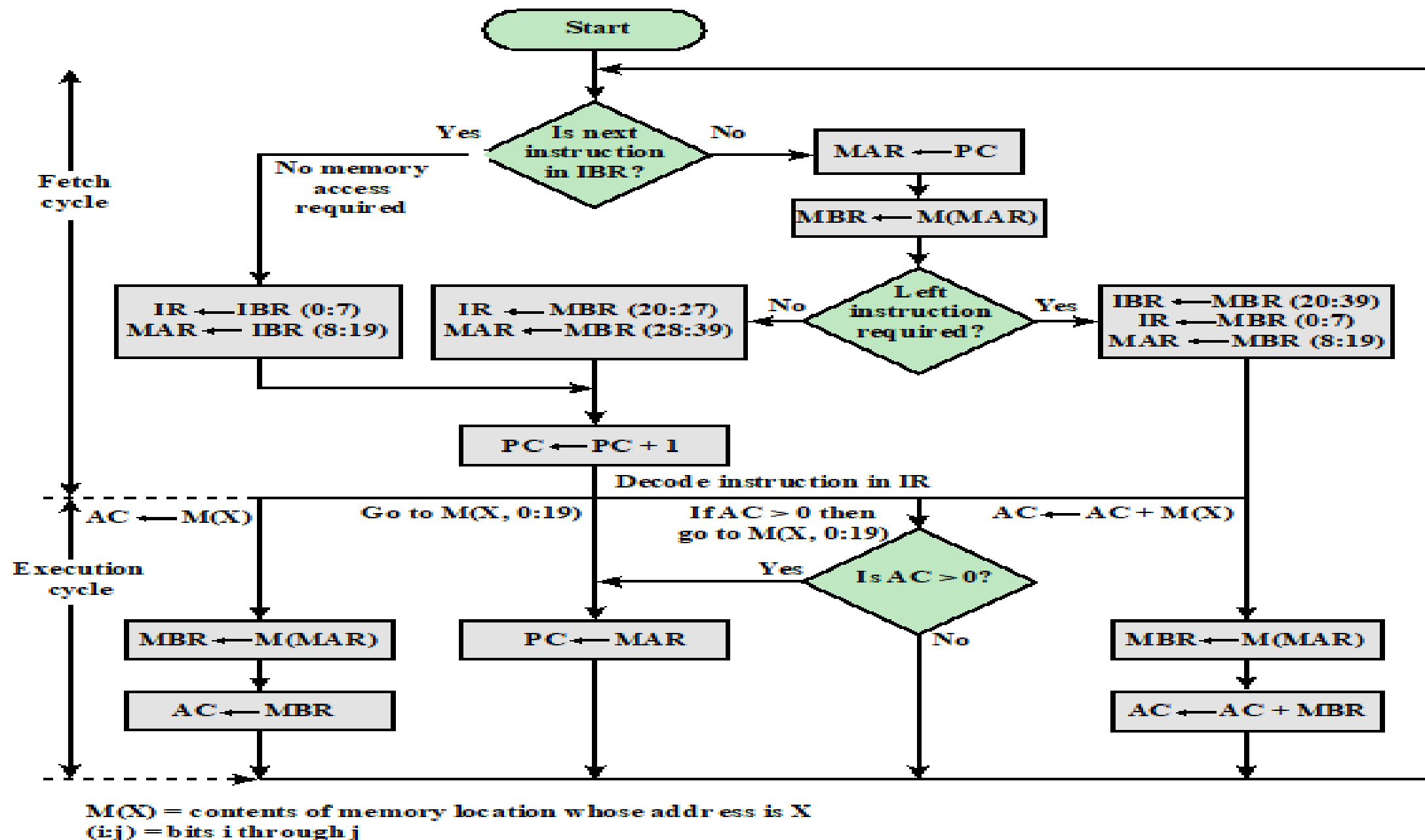
Partial Flowchart of IAS Operation
