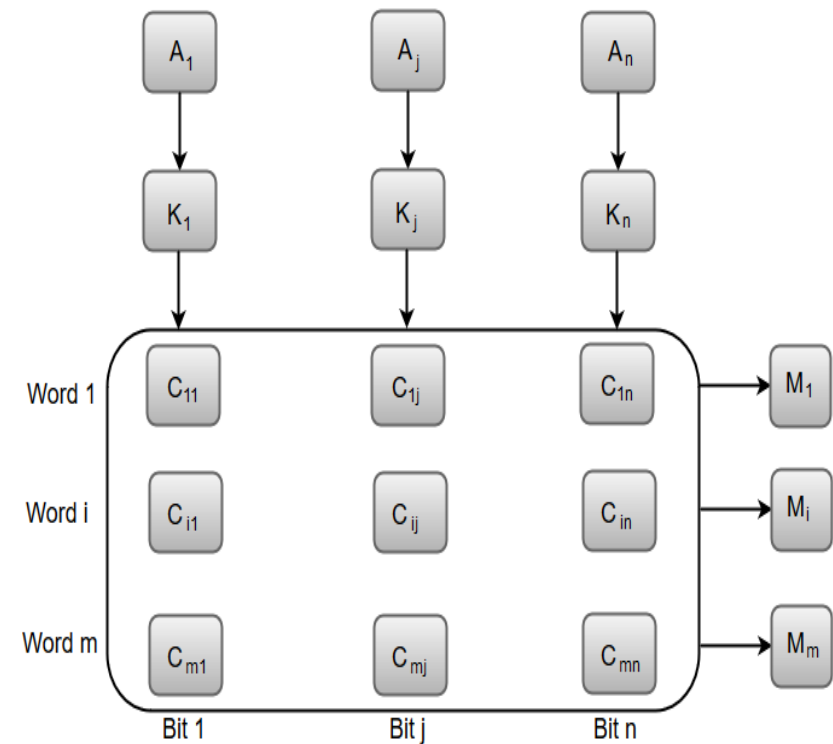
Associative memory of m word, n cells per word:
