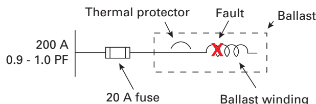
Figure 7.2.a UL 935 short-circuit test for ballast protectors.
