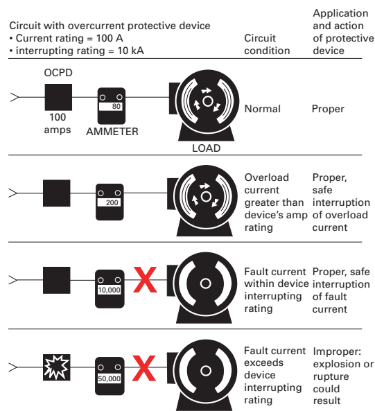
Figure 3.1.4.3.c Interrupting ratings are important for protecting against short-circuits.
