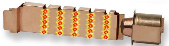
Figure 3.1.3.2.d Short-circuit element operation under fault conditions.
