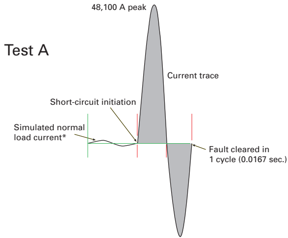
Figure 3.1.5.1.g Test A fault current waveform.
