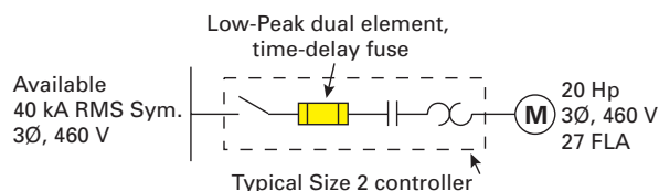
Figure 7.14.6.e Motor controller short-circuit protection
