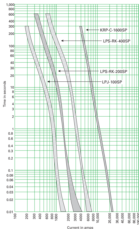
Figure 7.9.2.1.b A selectively coordinated system using fuses.
