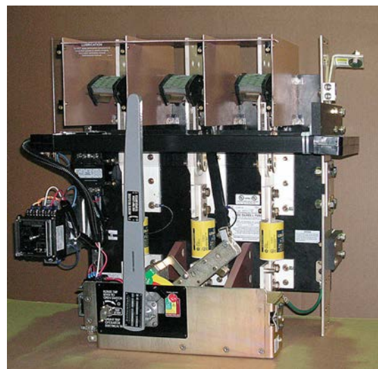
Figure 7.11.2.a Fusible bolted pressure switch equipped with ground fault protection relay and sensor. Courtesy of Boltswitch, Inc.
