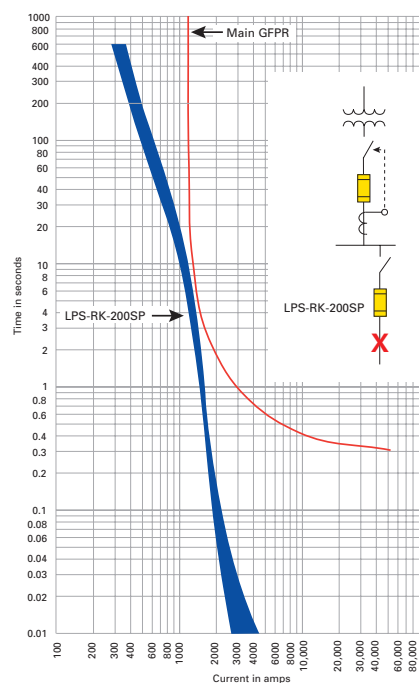
Figure 7.11.5.c Selective coordination considerations for low magnitude feeder ground faults. Longer GFPR delay permits larger feeder fuse to coordinate with main relay.
