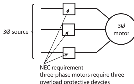
Figure 7.14.10.d Since 1971, the NEC has required three overload protective devices (one in each phase) for protecting three-phase motors.
