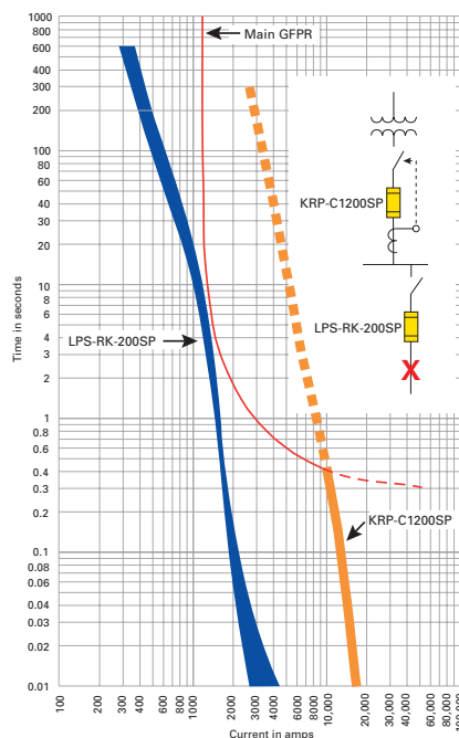
Figure 7.11.5.d Selective coordination considerations for high magnitude feeder ground faults involves analysis of main and feeder OCPDs. In this case the fuses are selectively coordinated so that an unnecessary blackout does not occur.
