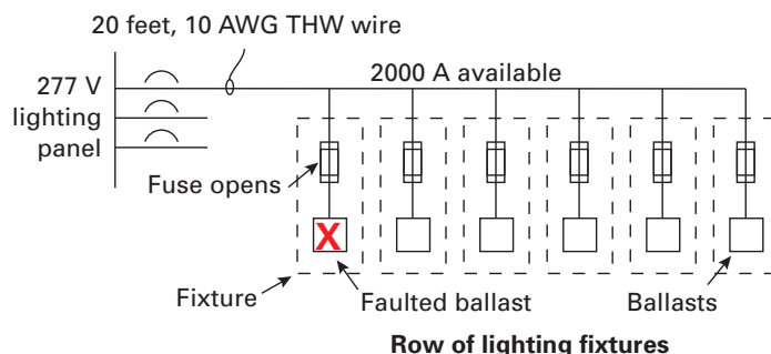
Figure 7.2.b Individual ballast fusing.
