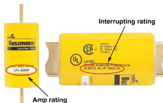
Figure 7.12.2.b Fuse with 300 kA IR at 600 Vac.
