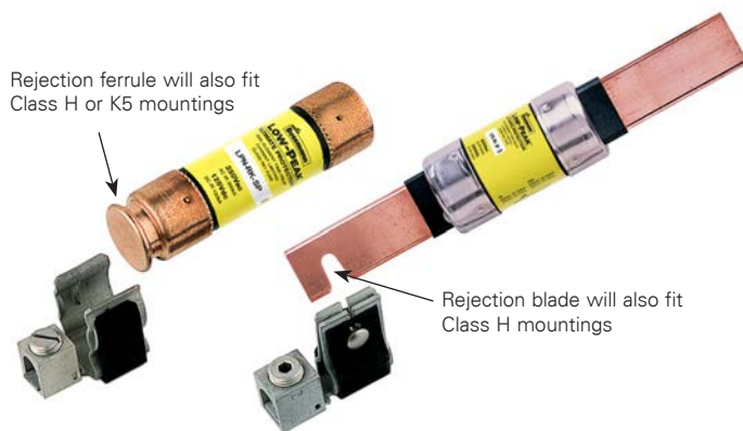
Figure 3.1.6.1.c Class R fuse rejection clips (restriction on the ferrule or notch on the blade) that will only accept Class R fuses.
