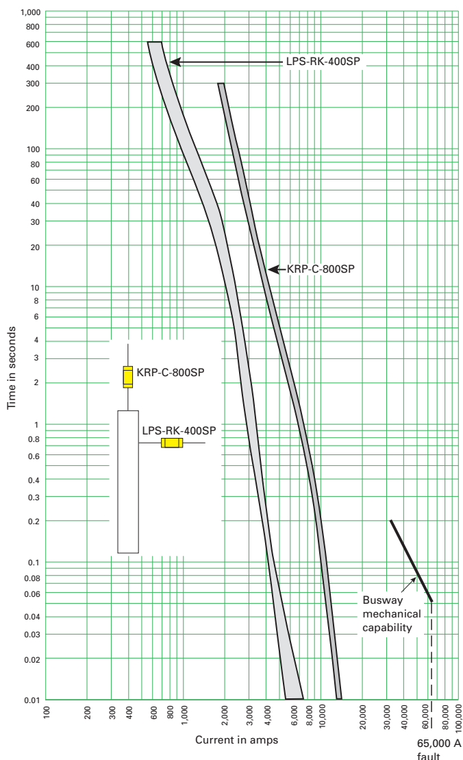
Figure 7.4.b Busway fault current protection with current-limiting fuses.
