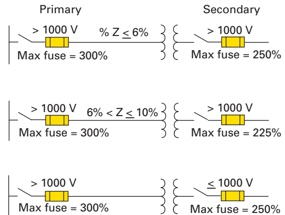
Figure 7.19.d Supervised locations
