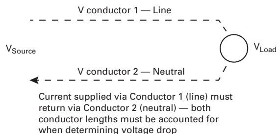
Figure 7.7.9.a Line and neutral conductors must both be considered for voltage drop calculations.
