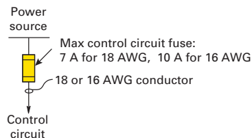
Figure 7.14.8.f Fuse amp limits for protecting 18 and 16 AWG control circuit conductors.
