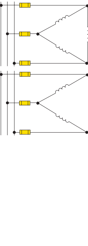
Figure 7.19.e E-Rated fuses for medium voltage transformers and feeders
