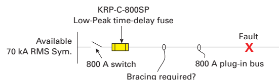
Figure 7.4.a Analysis of the short-circuit rating requirements.
