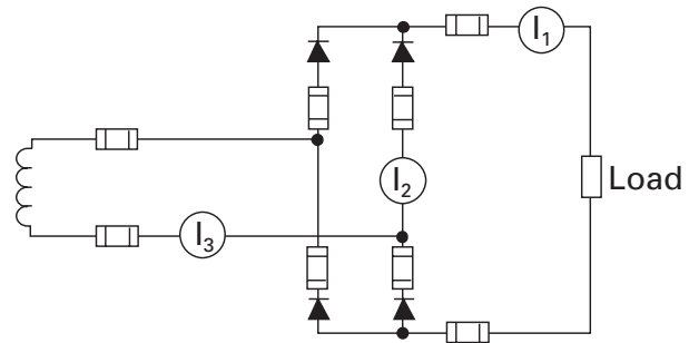
Figure 3.1.6.4.c Single-phase, full-wave, bridge.
