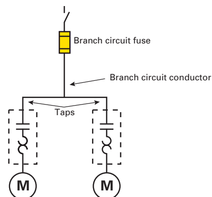
Figure 7.14.7.a Group motor installation (group fusing) NEC 430.53
