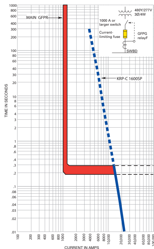
Figure 7.11.4.a "Effective" time-current curve for line-to-ground fault with a 1600 A fuse and GFPE set at 1200 A.
