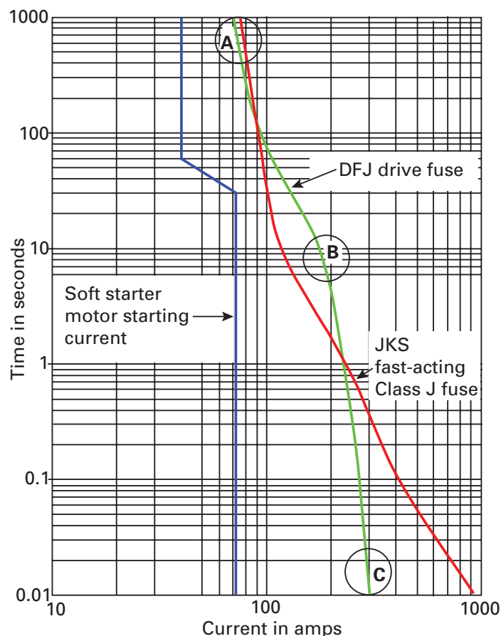
Figure 7.21.6.a Time-current characteristics comparisons show the DFJ's superior performance at three critical performance points.
