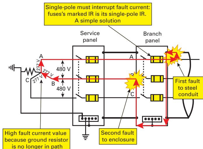
Figure 3.1.4.3.j The fault is essentially line-to-line with the conductors and ground path impedance.
