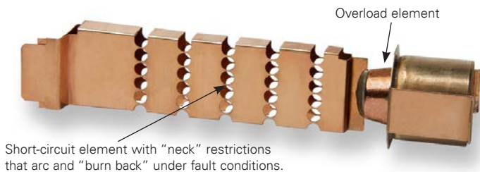
Figure 3.1.3.2.b “Dual-element” construction.
