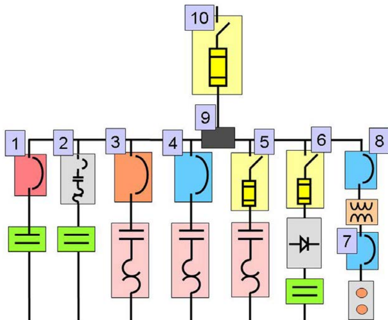
Figure 7.12.1.i Industrial control panel one-line diagram.
