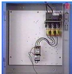
Figure 7.14.6.h: Using the same test circuit and starter as Figure 7.14.w during short-circuit interruption. The difference is current-limiting fuses provide the motor branch circuit protection. This illustrates the protection level required by UL 508E and IEC 60947-4-1 for Type 2 "No Damage" protection. The heaters and overload relays maintained calibration, retaining the extremely important circuit overload protection. This starter could be put back into service without any repair.
