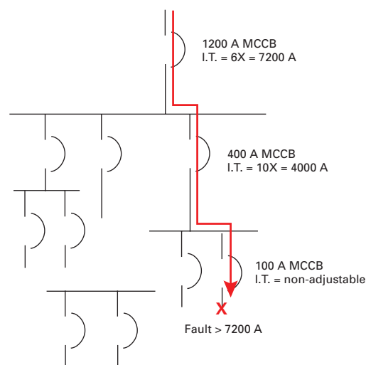
Figure 4.2.6.3.a shows a one-line diagram with three molded case circuit breakers in series: 1200 A main, 400 A feeder and 100 A branch circuit. The other circuit breakers on the one-line diagram supply other circuits and loads. The fault current path from the power source is depicted by the red arrow/line. For the coordination analysis, faults on both the branch and feeder circuit must be analyzed.
