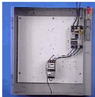
Figure 7.14.6.f: Before test with an OCPD that only provides Type 1 protection as motor branch circuit protection for 10 Hp, IEC starter with 22 kA available at 480 V.
