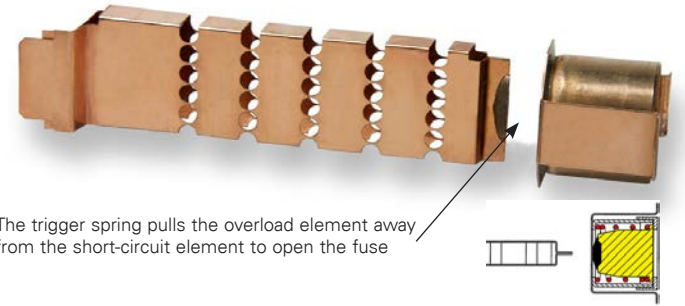
Figure 3.1.3.2.c Overload element operation.
