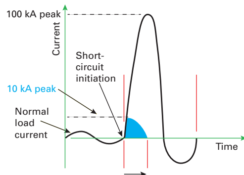
Current limiting fuse opens and clears short-circuit in less than 1/2 cycle
