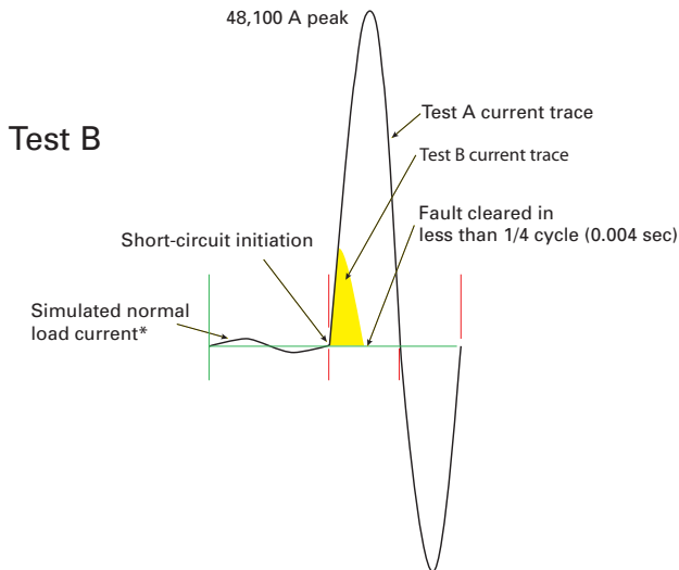
Figure 3.1.5.1.h Test B fault current waveform.
