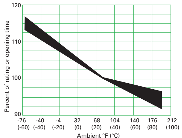
Figure 3.1.3.2.j Ambient temperature single-element derating curve.
