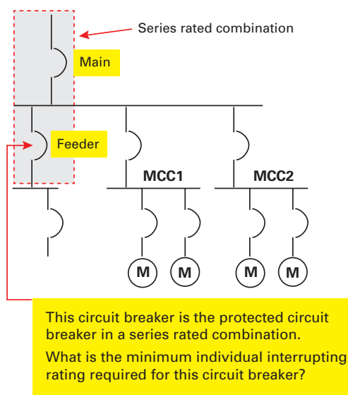
Figure 7.6.7.a Example 1 diagram.
