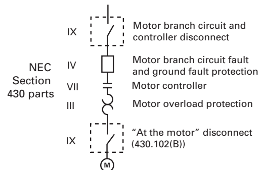
Figure 7.14.a NEC 430 parts.
