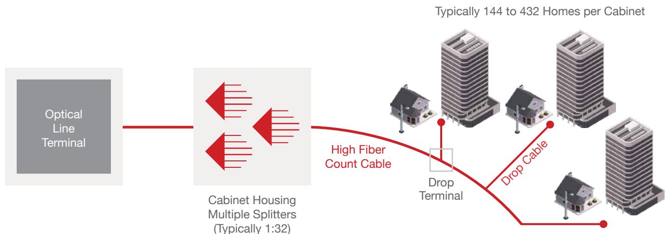
FIGURE 5: Centralized Splitting
