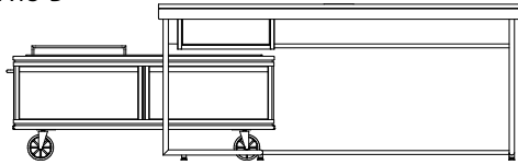
Left Desk Wall Unit 98 3/32 x 24 x 30 overall
