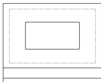
TV Panel 3855A62AXX SG-205.1 53 x 5 x 42 1/2
