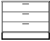
Dresser 3855B01DXX SG-230.1 42 x 15 3/4 x 34
