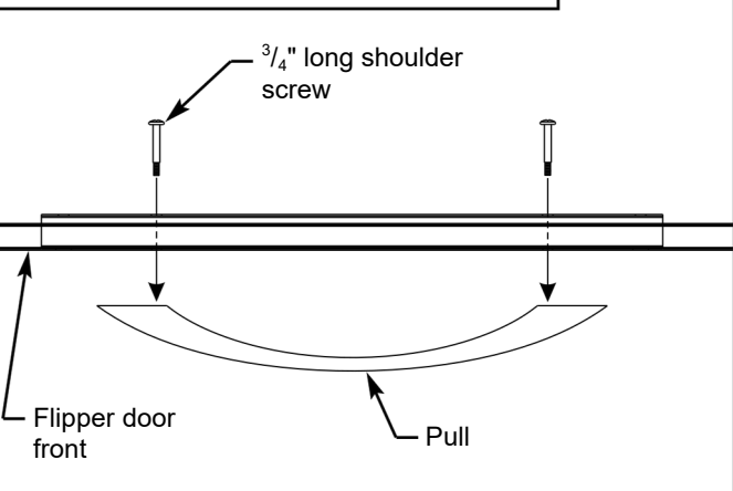
Illustration 2. Flipper Door Pull Installation:
