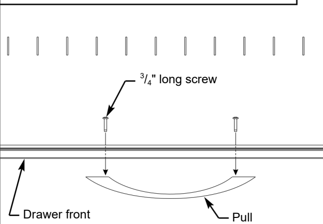
Illustration 3. Fixed Front Drawer Pull Installation:
