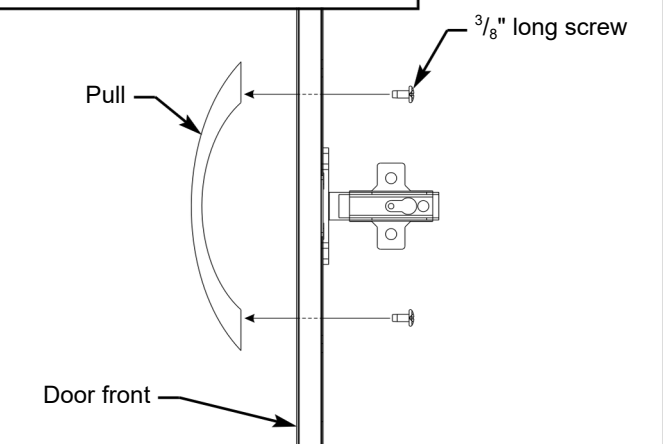
Illustration 4. Door Pull Installation:
