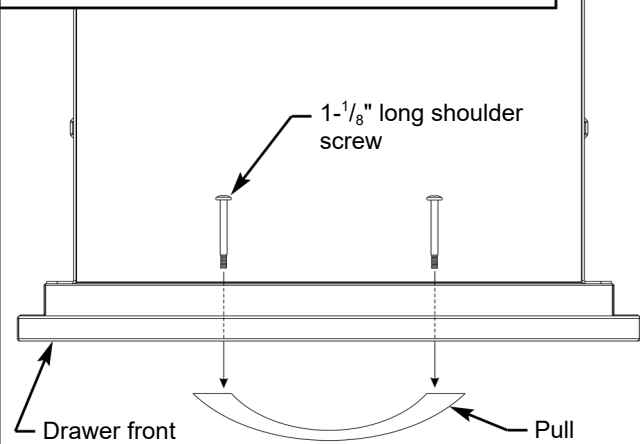
Illustration 1. Pedestal Drawer Pull Installation:
