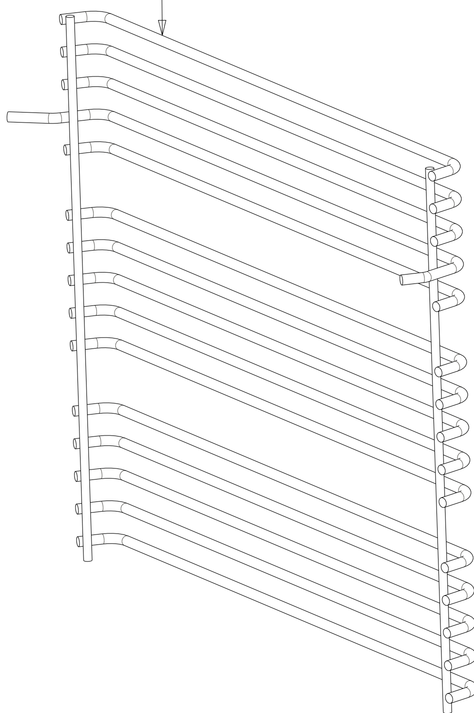
ALTERNATIVE SHELF GUIDES- KEY NUMBER FOR OPPOSITE HAND 421
