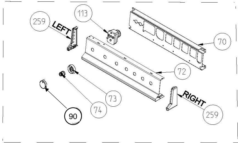
MECHANIC TIMER (OPTIONAL)
