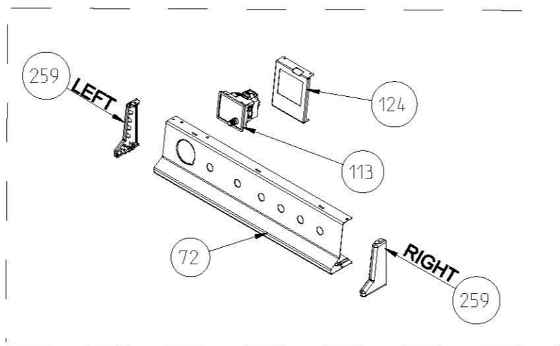
ANALOG TIMER (OPTIONAL FOR 60X60)
