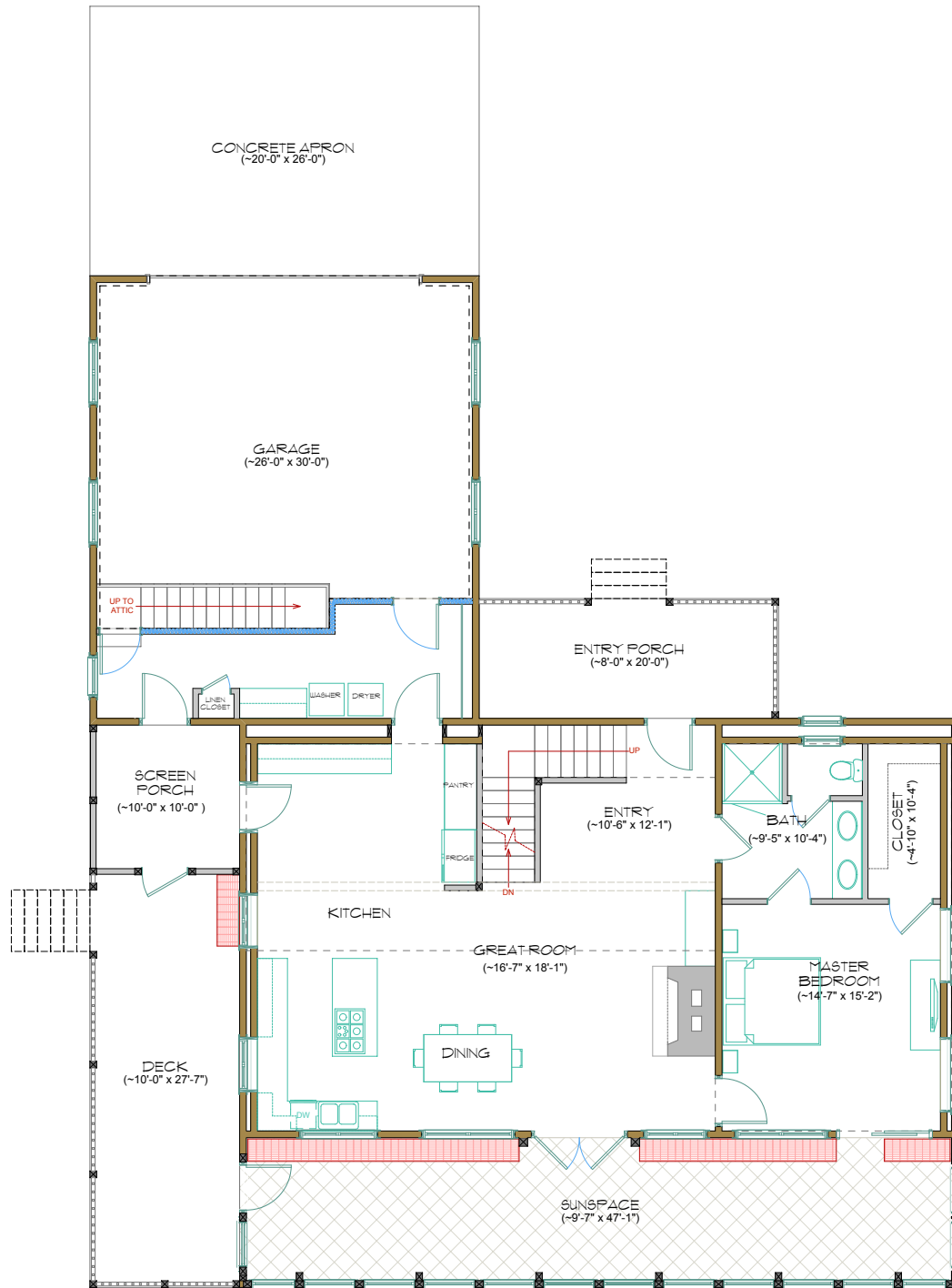
MAIN LEVEL - 2006 SQ.FT.
