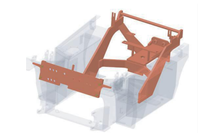
Reinforced frame
