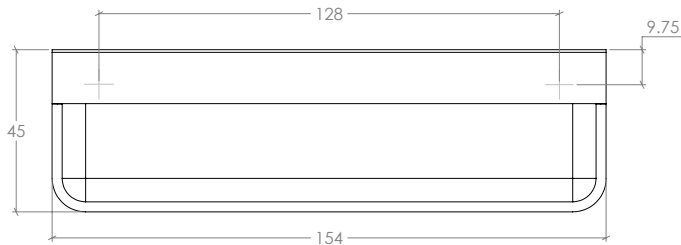
Flush Pull Handle
