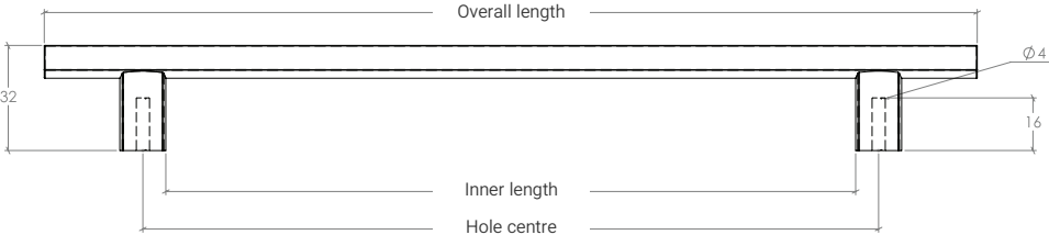
D Handle
