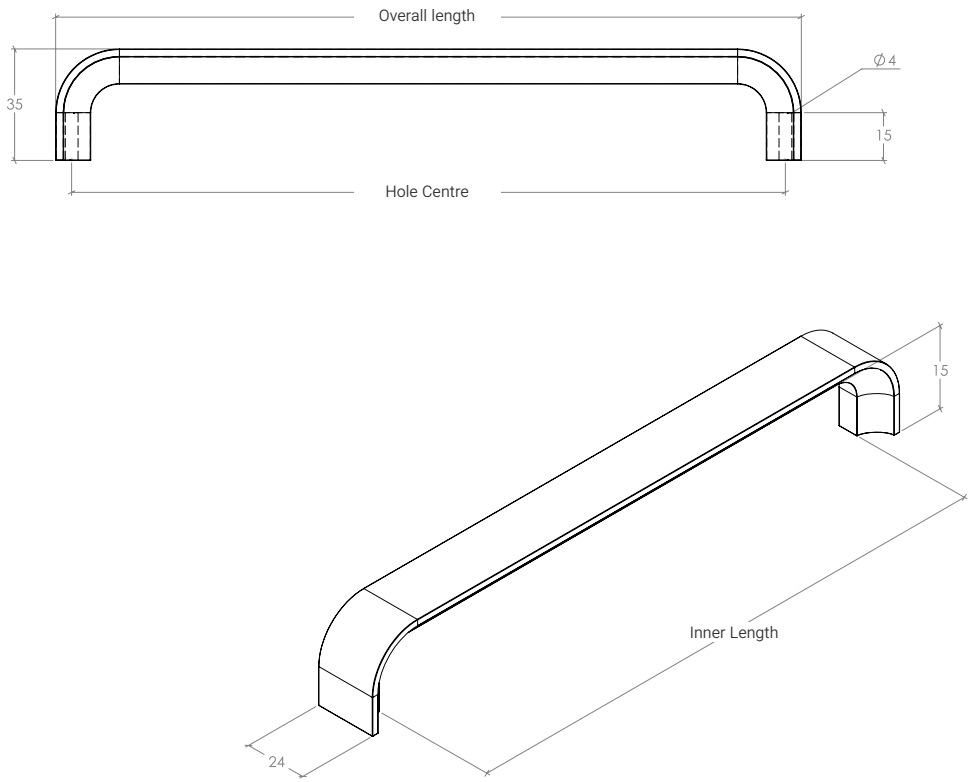
D Handle
