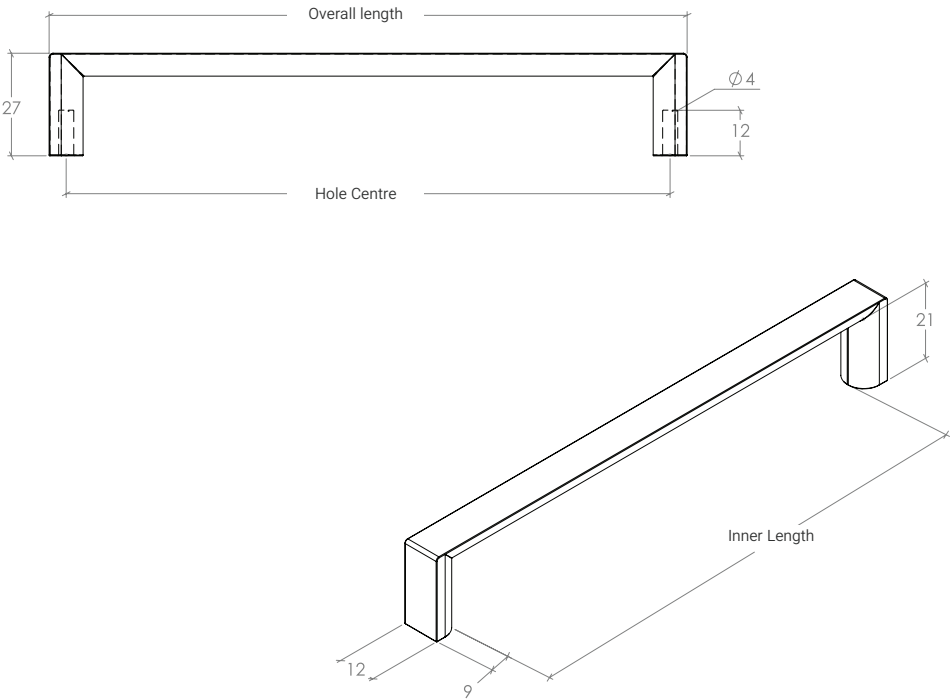
D Handle
