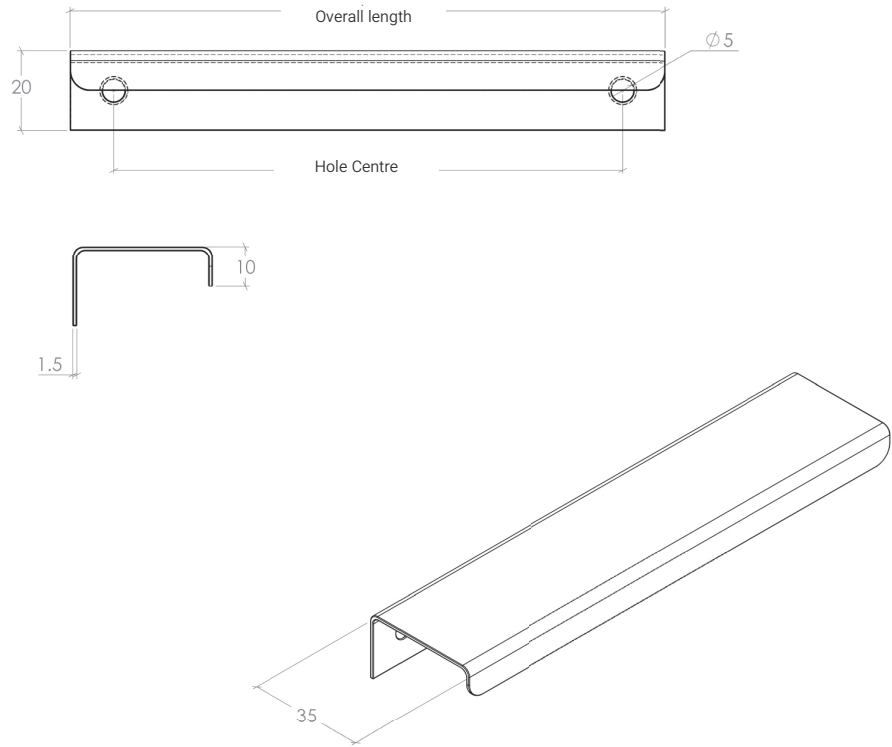
Lip Pull Handle
