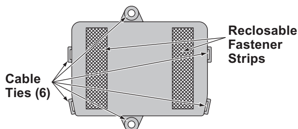
Isolation Module (bottom view)
