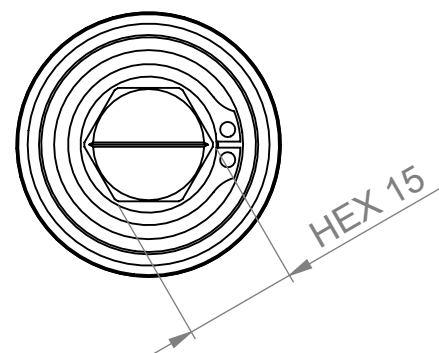
Top view of the stem without the plug
