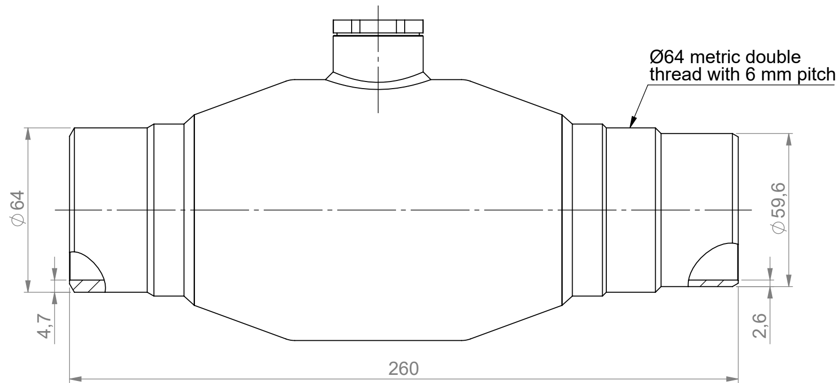
Top view of the stem without the plug
