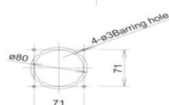
Dimension of Fresh air intake duct (field supply) connection port
