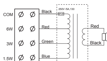
Cable configuration
