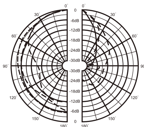
Polar Diagram
