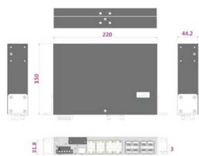
IES2000-TW8S8P
