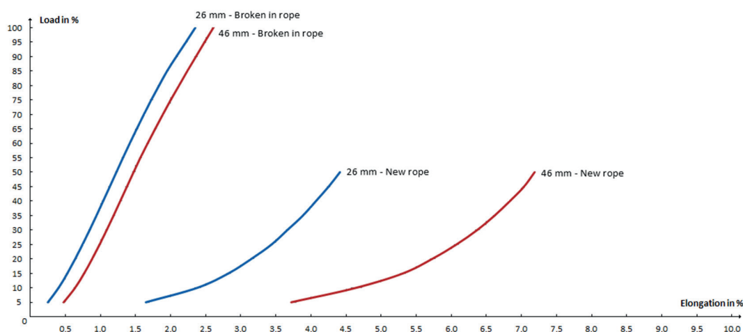
Examples of elongation for new and broken in rope - 26 mm and 46 mm
