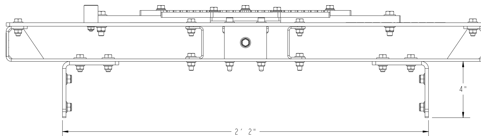
2' 2" Max Inside Bed Rail Spacing For Alternate Mount (recommended, not required)
