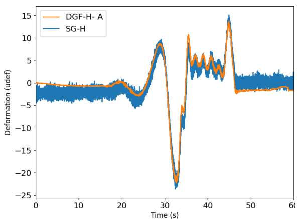
Figure 7: Dragonfly® (DGF) and SG signal while 2 trains pass on the bridge (Train 1 and 2)
