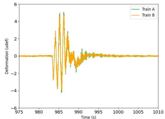
Figure 9: Dragonfly® (DGF) for 2 different passenger trains coming from the train station. Train B time has been shifted for superposition.
