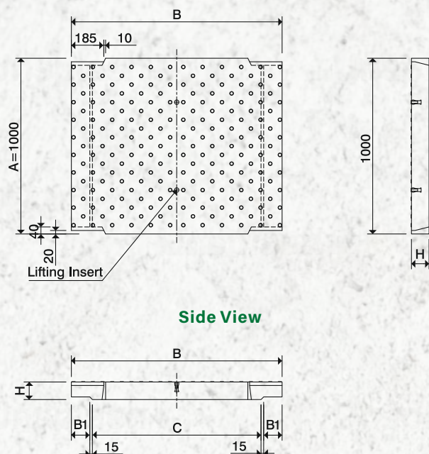
TOP VIEW STD. Lid For SWD
