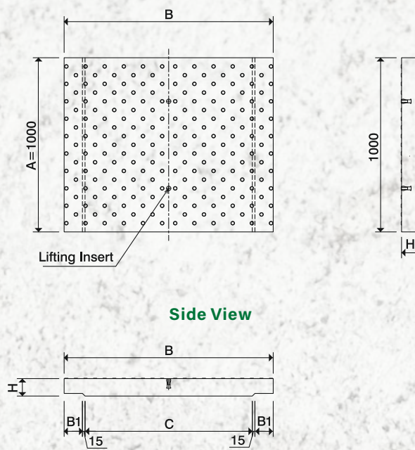
TOP VIEW No Hole Lid For Cable Duct
