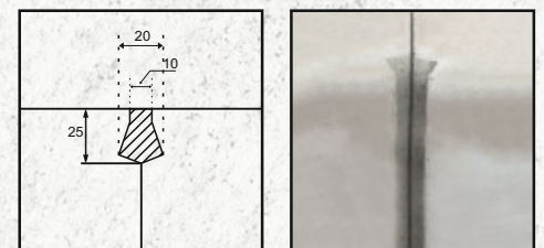
Typical Groove For Joint
