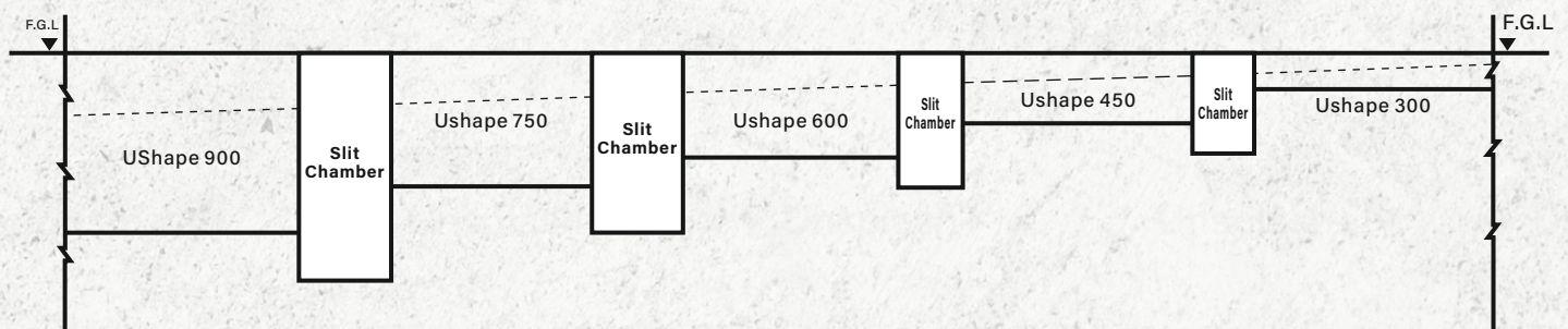
Typical Cross Section For Slope
